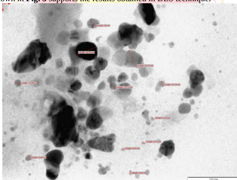
Fig.3 : Microphotograph of AgNPs obtained by TEM
