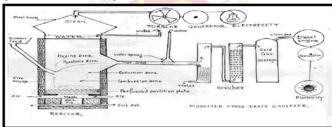
Figure : Modified Cross Draft Gasifier (Proposed)
