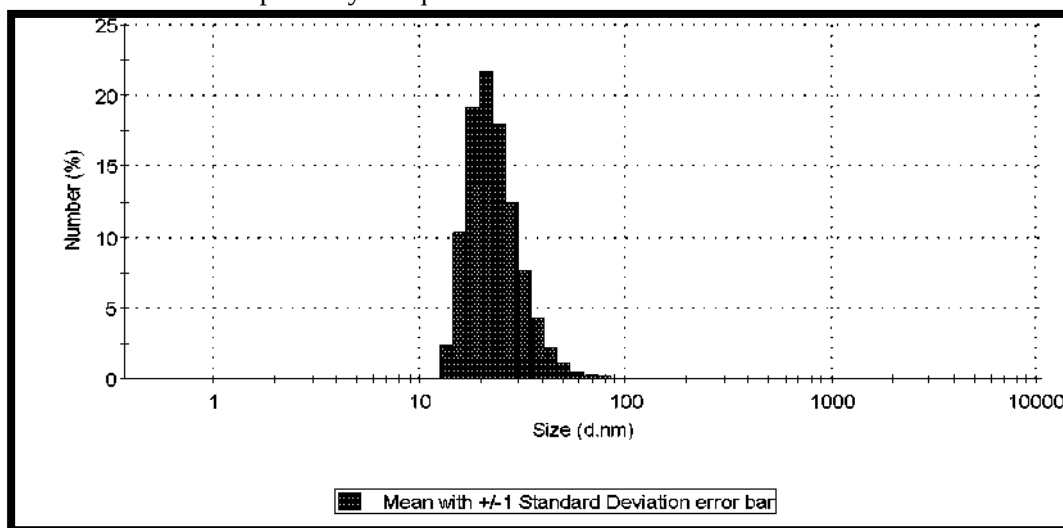
Fig. 2: Particle size distribution of AgNPs obtained using DLS equipment
